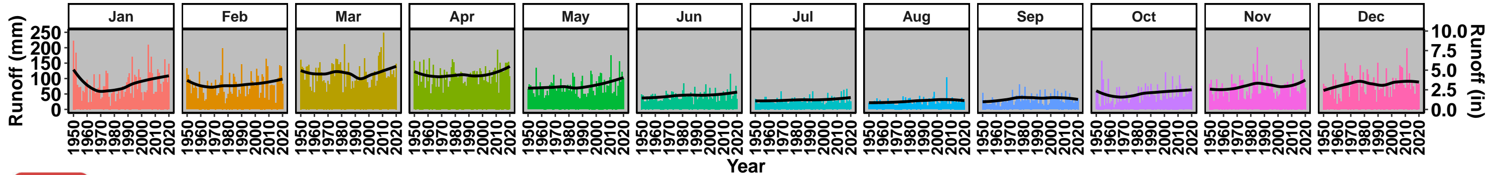
Lake Erie Monthly Runoff
