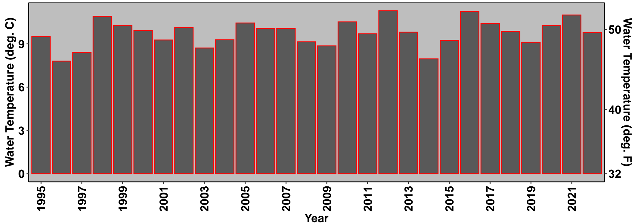
Lake Michigan Annual Average Surface Water Temperature
