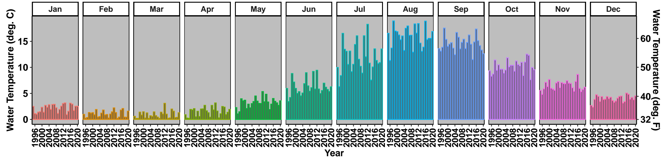
Lake Superior Monthly Average Surface Water Temperature
