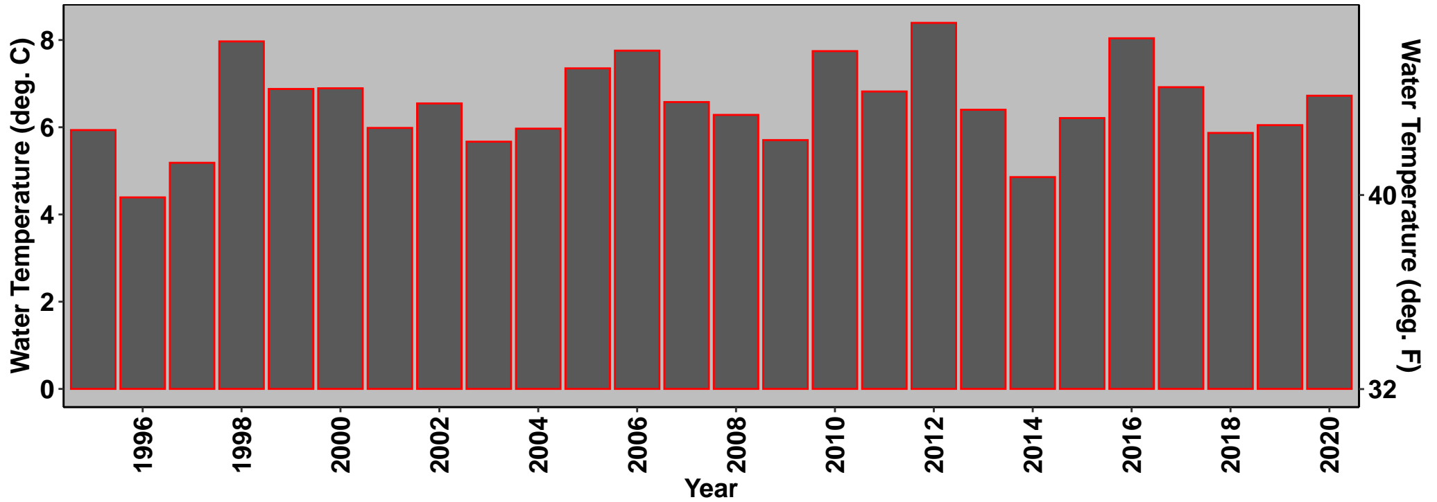
Lake Superior Annual Average Surface Water Temperature
